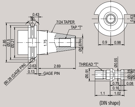
CAT40 Unit : in.
